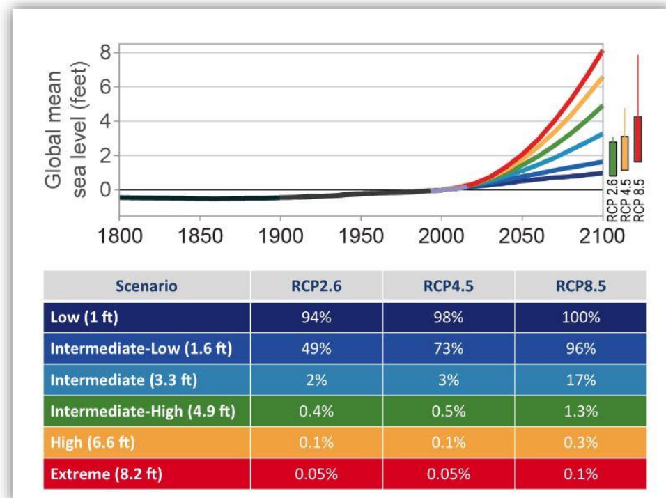
Figure 1: Global Mean Sea Level Rise (1800-2100)
