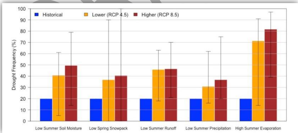
Figure 3: Drought Metrics for Clatsop County
